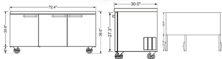
Dimensions (W" x D" x H") 72.4 x 30 x 36
