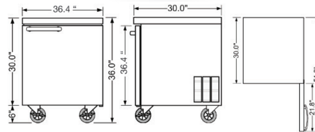
Dimensions (W" x D" x H") 36.4 x 30 x 36
