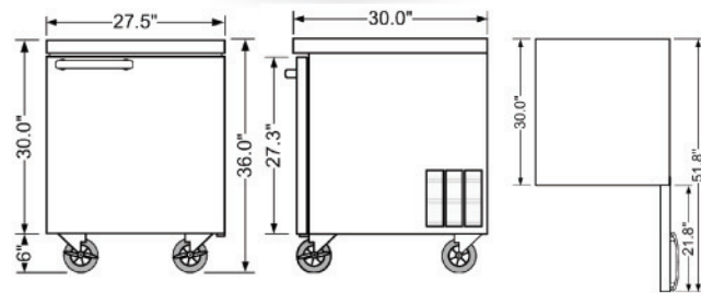
Dimensions (W" x D" x H") 27.5 x 30 x 36
