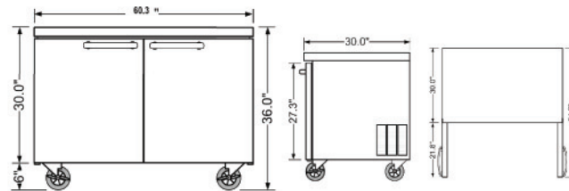
Dimensions (W" x D" x H") 60.4 x 30 x 36
