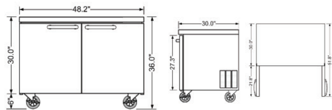
Dimensions (W" x D" x H") 48.3 x 30 x 36
