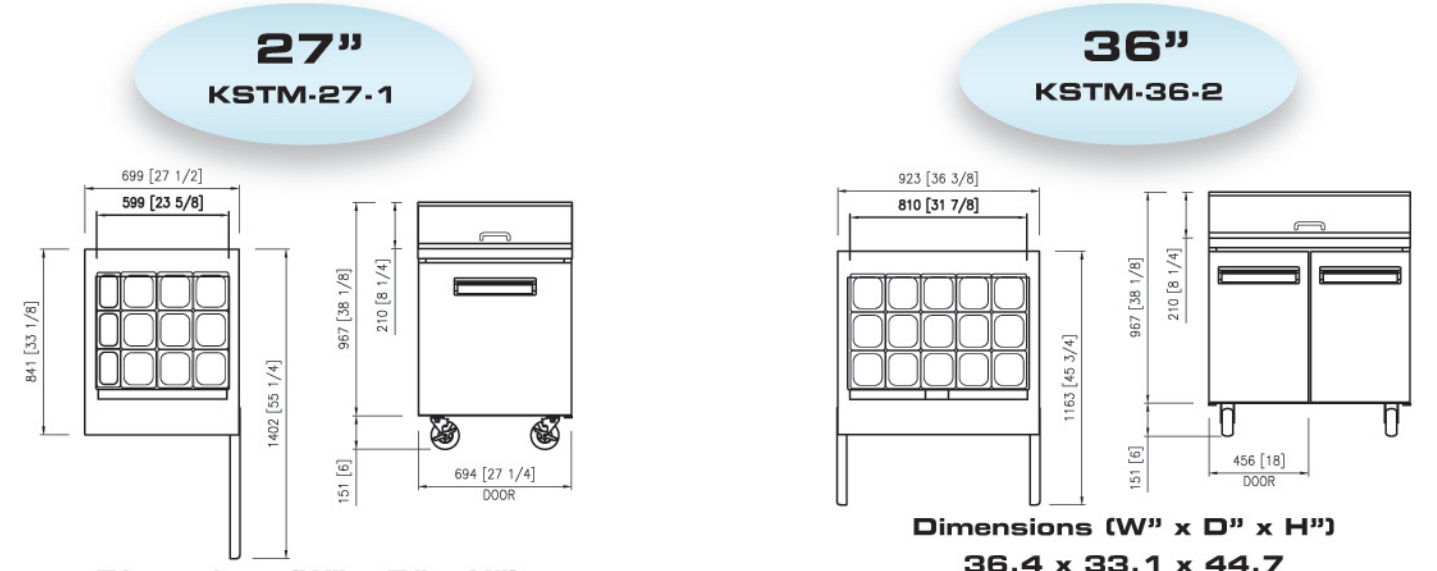
Dimensions (W" x D" x H") 27.5 x 33.1 x 44.7
