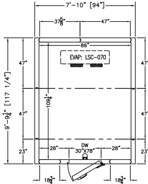
PLAN VIEW
