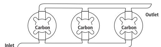
ex. Triple Head Parallel Flow
